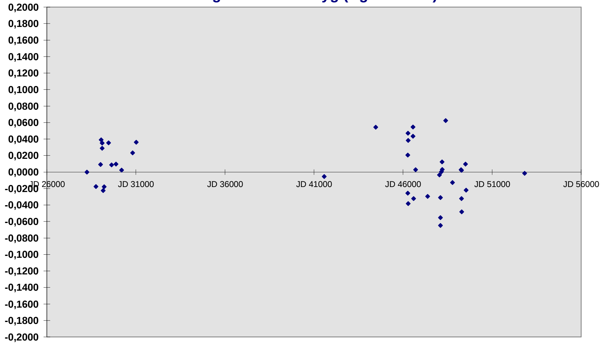
O-C diagram of V513 Cyg (Ag/MS 1991)
